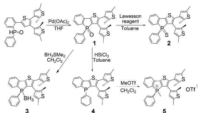
Scheme 1. Synthesis of 1–5.
